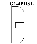
Round screw head G1-4 with body 100 mm long - lateral
