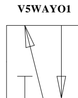
5 way valve open type 1 (P-A and B-S)
