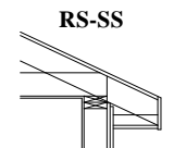
Roof Section with Short Soffit.
