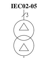
3 phase, 3 winding transformer with Delta-Delta connection
