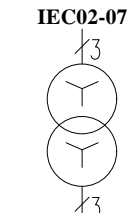
3 phase, 3 winding transformer with Wye-Wye connection
