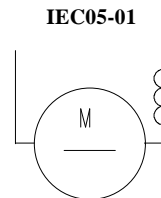
Motor direct current, in series excitation
