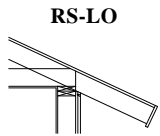
Roof Section with Long Overhang.
