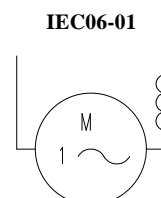
1-phase alternating current motor, in series excitation
