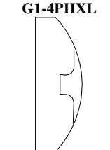
Philips round screw head G1-4 with body 100 mm long - lateral
