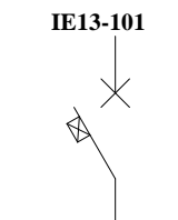
Power switch with automatic breaking
