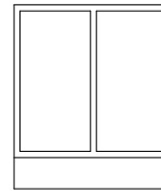
Base Cabinet 2 Doors 70x80
