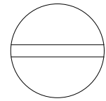
G516FS82 Screw head G5-16 with body 82 mm long - front
